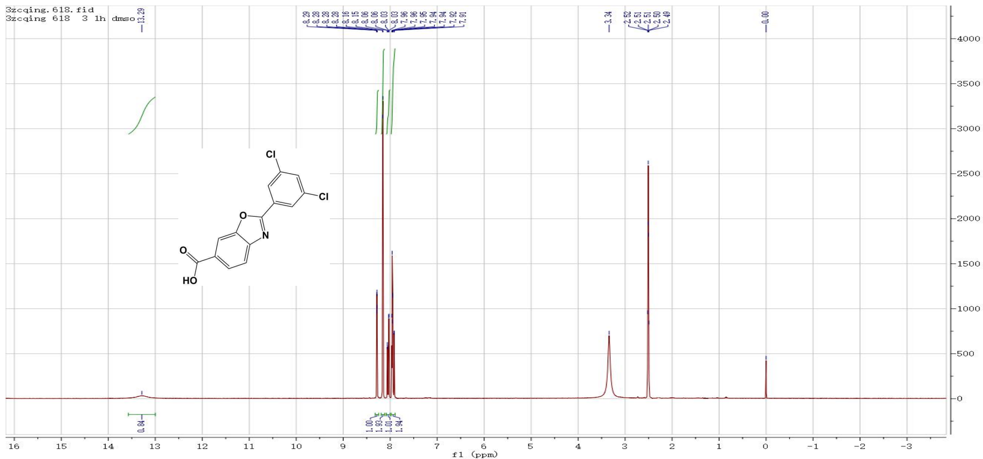
Tafamidis 594839-88-0 1HNMR Spectrum
