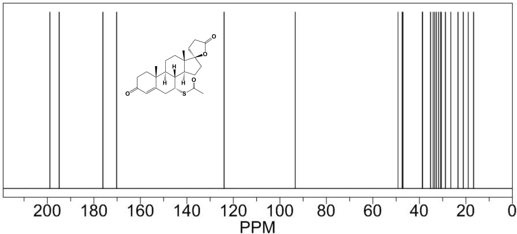
Spirolactone (Cas 52-01-7) 13 CNMR Spectrum
