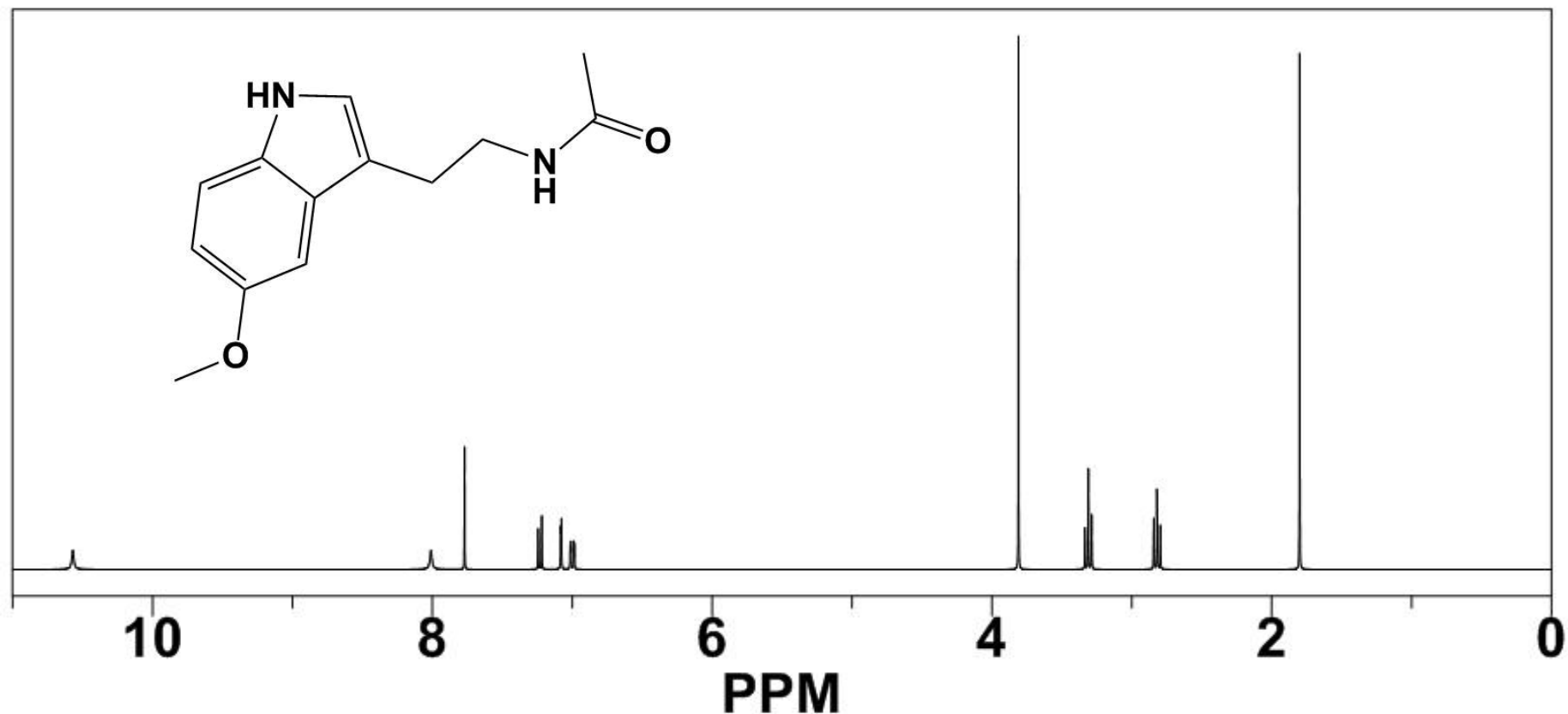
Melatonin 73-31-4 1 HNMR Spectrum
