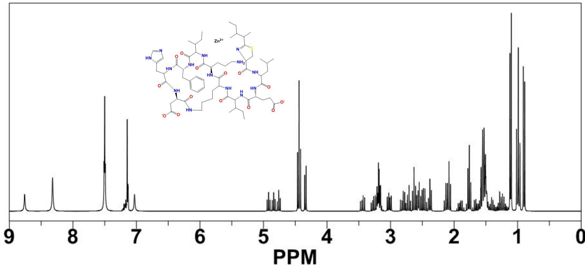
Bacitracin Zinc Cas 1405-89-6 1HNMR Spectrum
